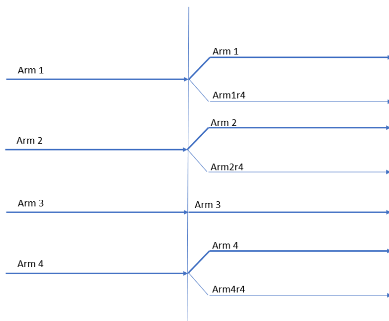
Figure 1: Randomisation diagram
