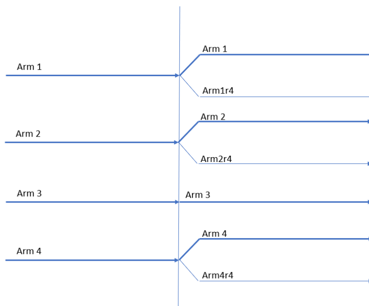
Figure 1: Randomisation diagram
